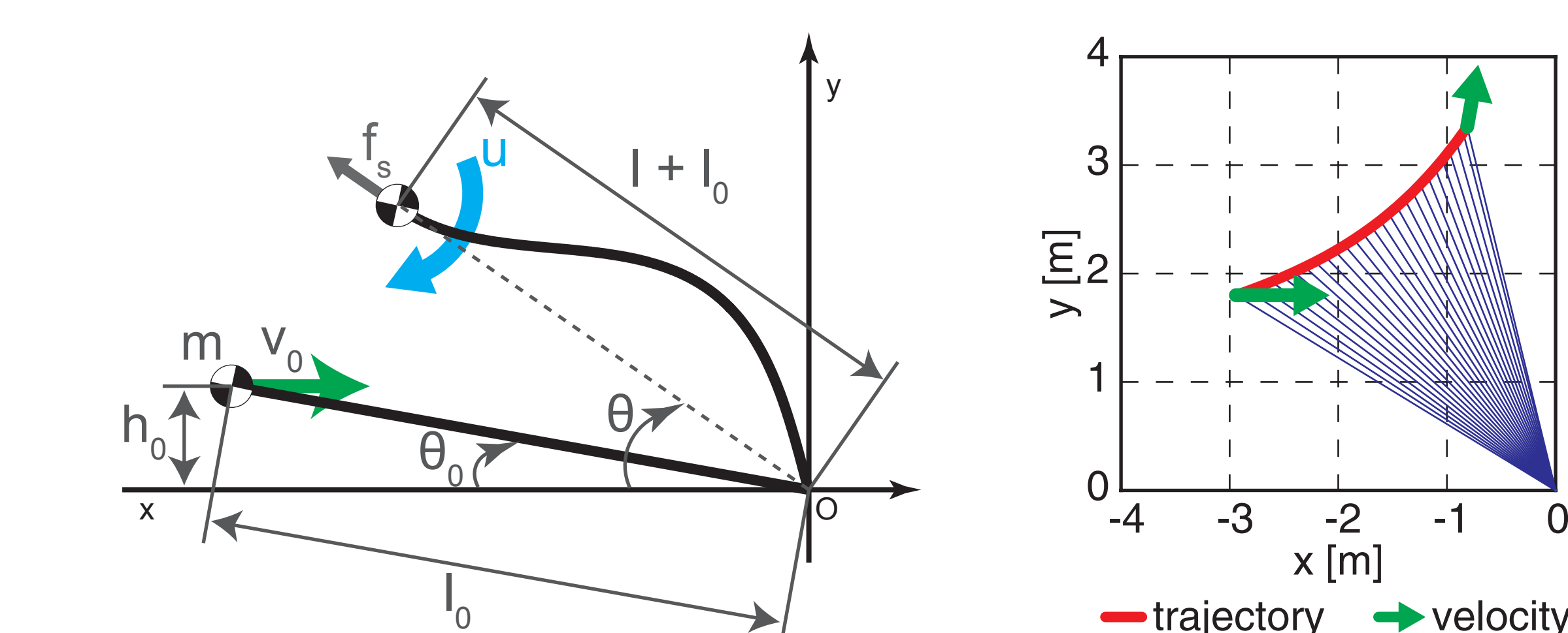
Fig2. Simulation model
