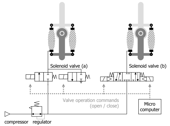
Fig. 3. Pneumatic and electric system
